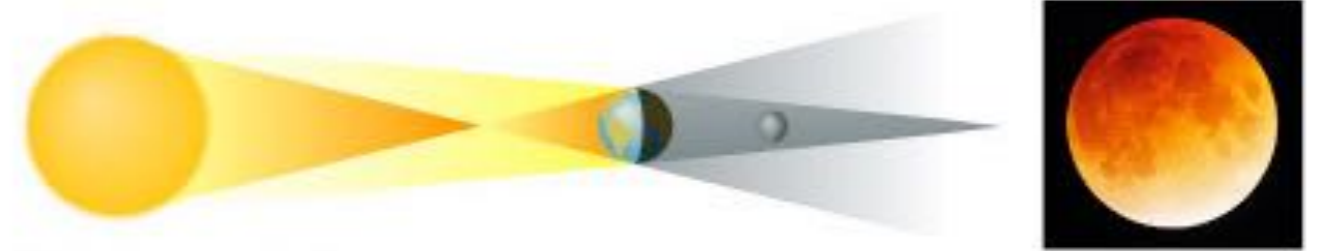
Total Lunar Eclipse
