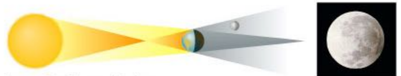
Penumbral Lunar Eclipse
