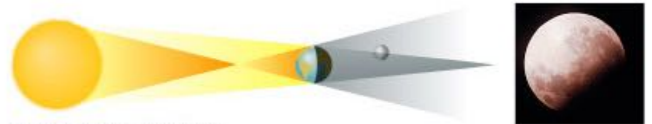
Partial Lunar Eclipse
