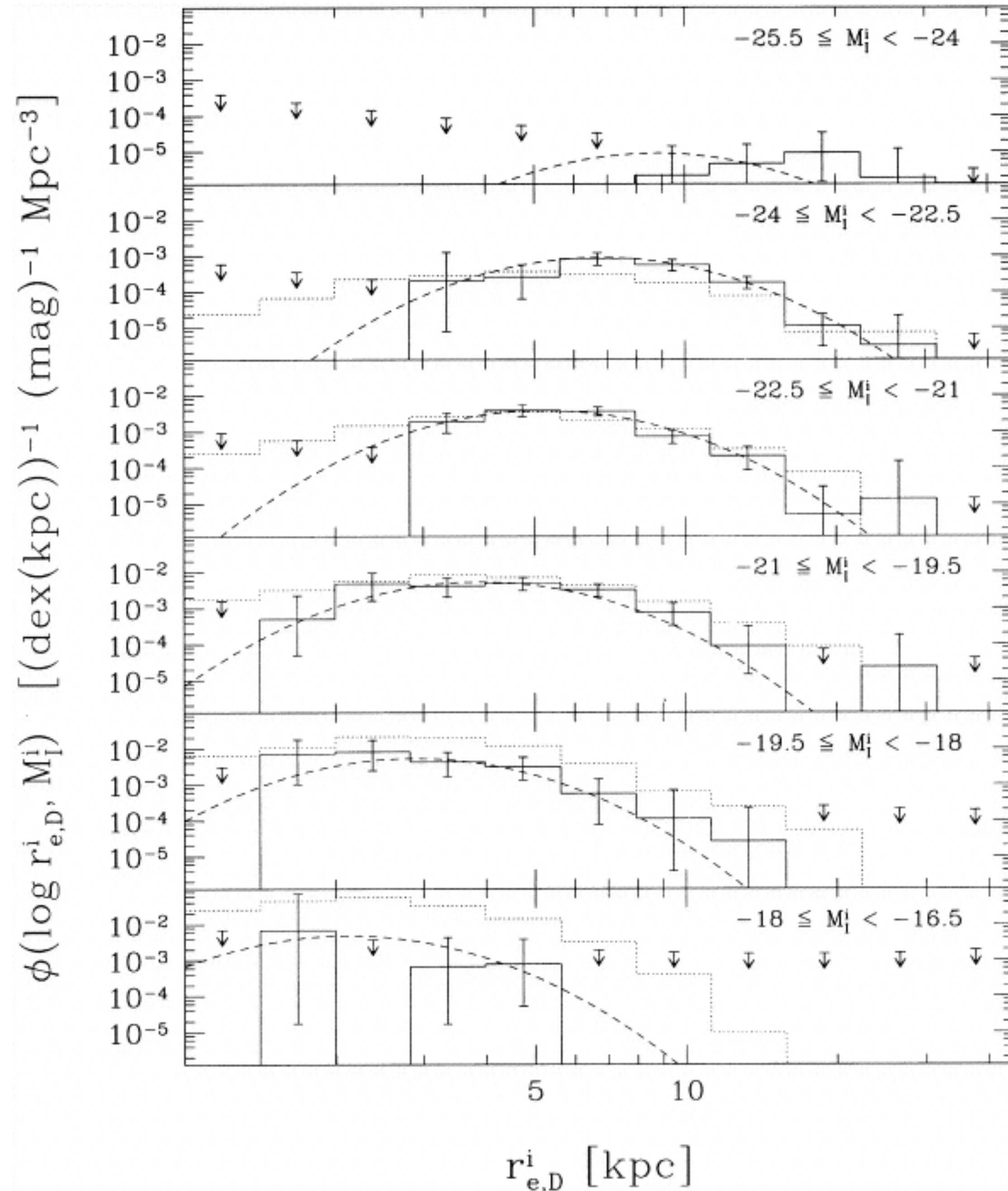
Bivariate distribution of luminosity and size (de Jong & Lacey 2000)
