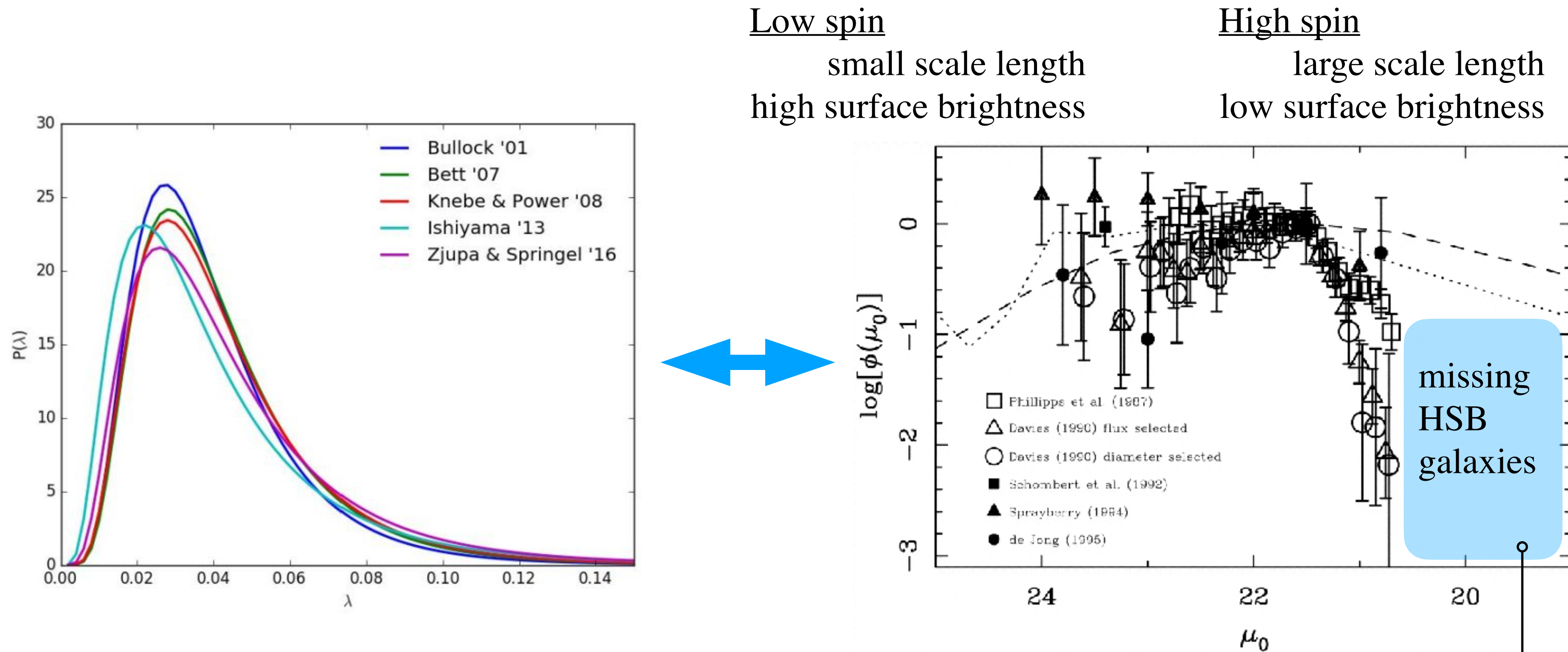
McGaugh & de Blok (1998); see also Mo, Mao, & White (1998)
